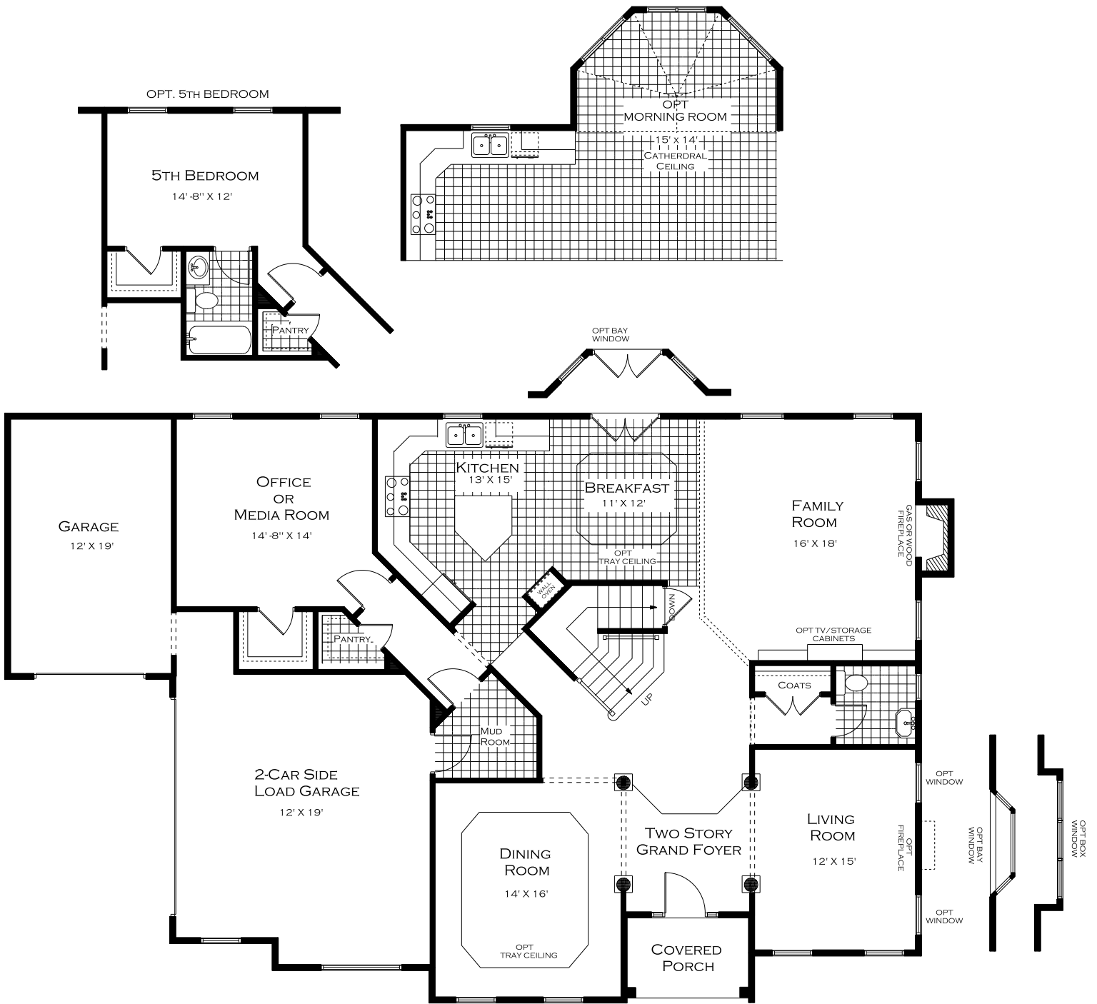
THE PARK AVENUE MAIN FLOOR PLAN 1,856 SQ. FT.
