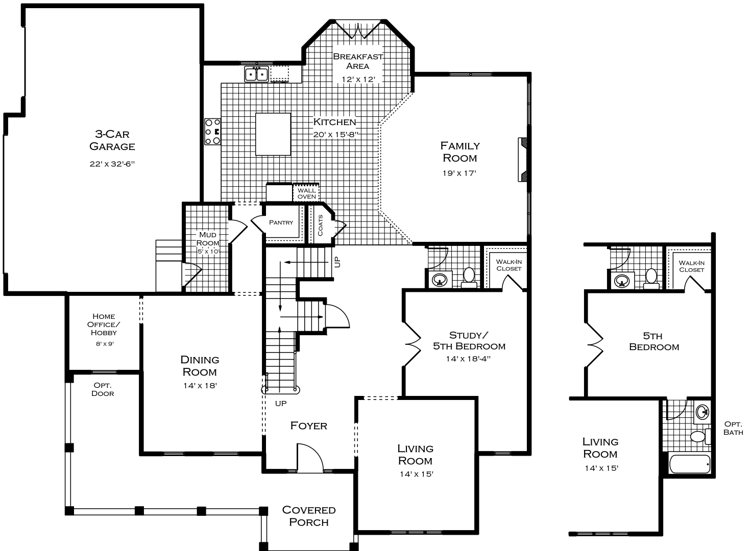
THE NEW HAVEN FIRST FLOOR PLAN 2,100 SQ. FT.
