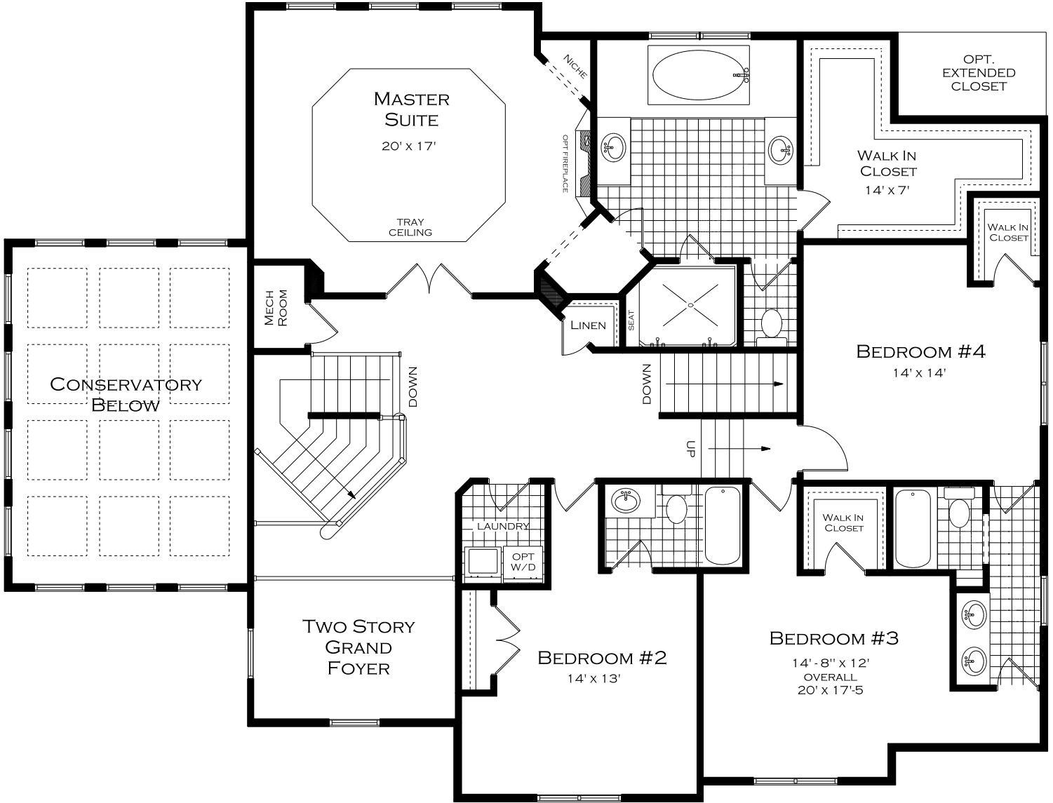
THE EVERGREEN SECOND FLOOR PLAN 1,911 SQ. FT.
