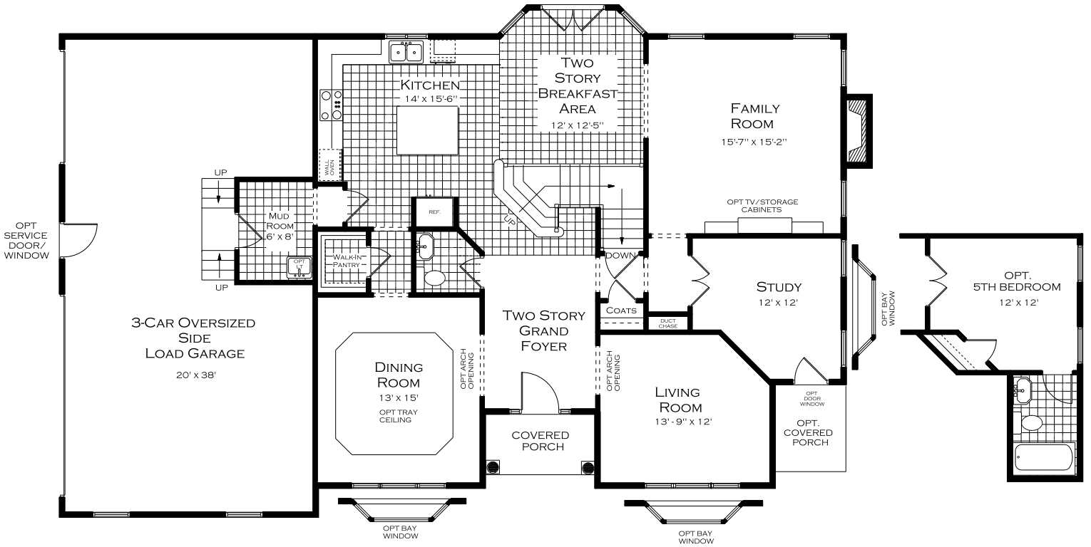
THE CARMICHAEL MAIN FLOOR PLAN 1,540 SQ. FT.
