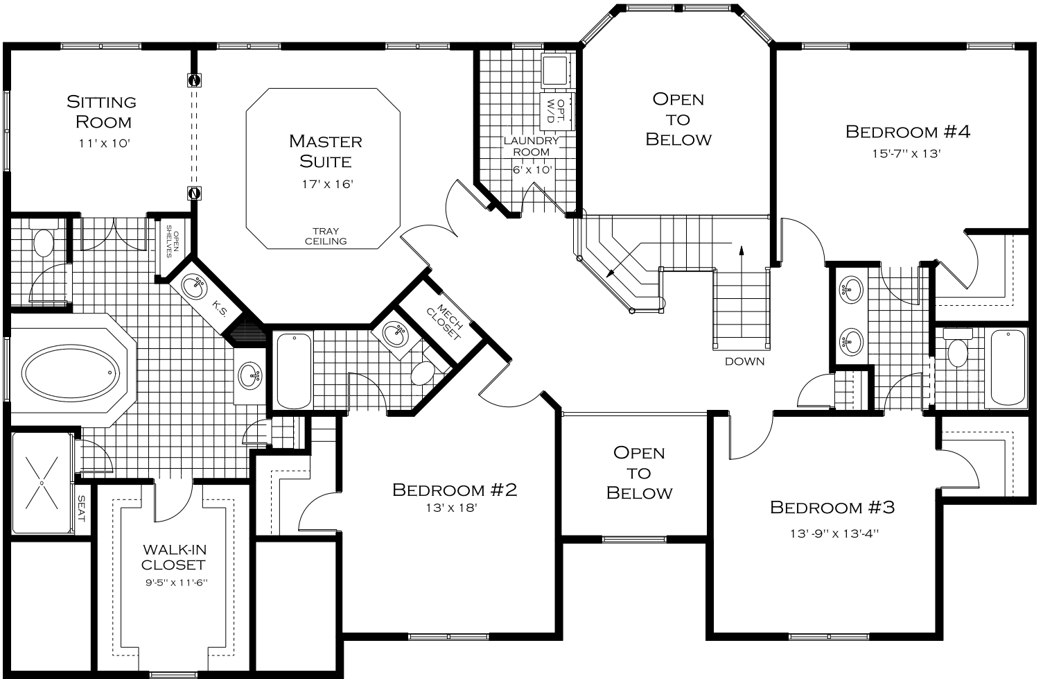
THE CARMICHAEL SECOND FLOOR PLAN 1,966 SQ. FT.
